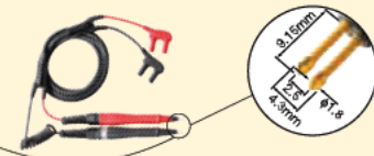
PIN TYPE LEAD 9465-10 A: 80 mm (3.15 in) (Red), 140 mm (5.51 in) (Black, Max. 550 mm (21.65 in)), B: 121 mm (4.76 in), L: 1.88 m (6.17 ft)
