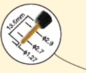
PIN TYPE LEAD 9465-10 A: 80 mm (3.15 in) (Red), 140 mm (5.51 in) (Black, Max. 550 mm (21.65 in)), B: 121 mm (4.76 in), L: 1.88 m (6.17 ft)
